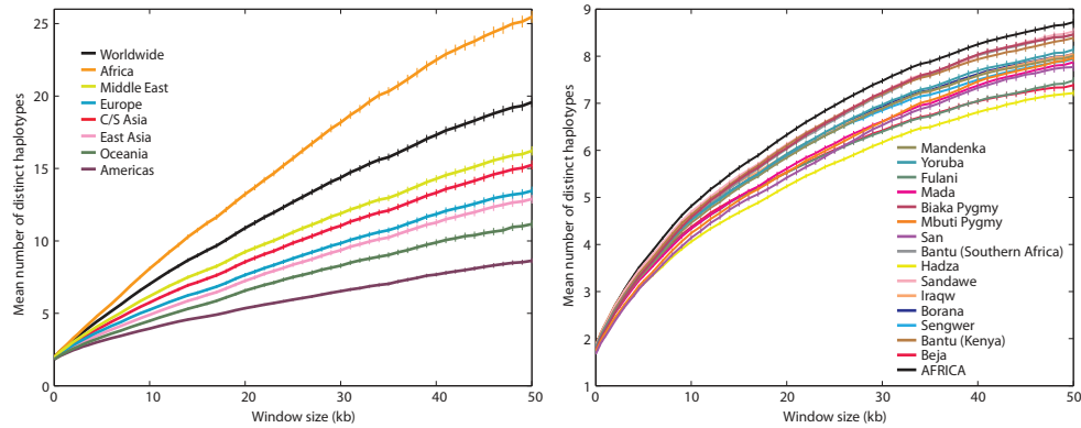
Figure S1: Numbers of distinct haplotypes. (A) The number of distinct haplotypes in each geographic region, and in the pooled worldwide collection, as a function of haplotype length. Sample sizes were adjusted to represent 54 chromosomes from each geographic region. (B) The number of distinct haplotypes in each African population, and in the pooled African population, as a function of haplotype length. Sample sizes were adjusted to represent 12 chromosomes from each population. Error bars represent the standard error of the mean across haplotype-loci.
